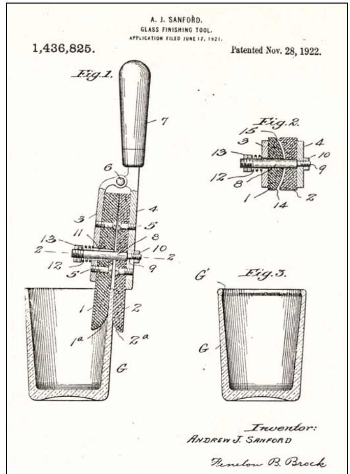
Patent 1,436,825
