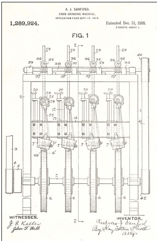
Patent 1,289,924 – Illustration 1
