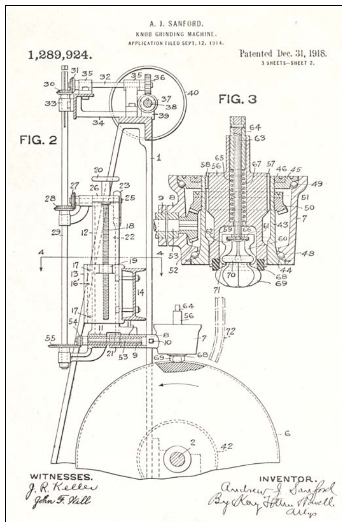
Patent 1,289,924 – Illustration 2
