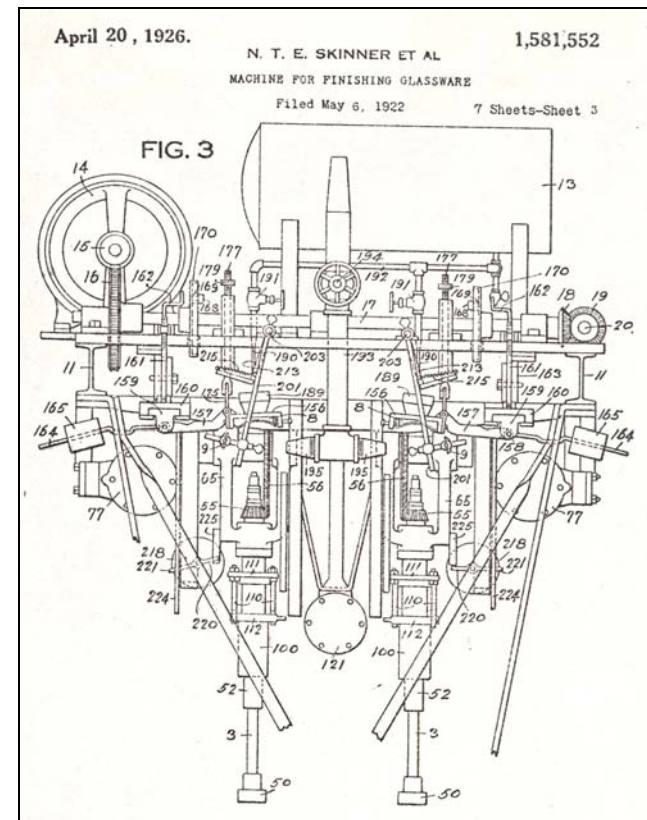
Patent 1,581,552 – Illustration 3
