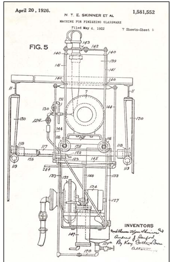
Patent 1,581,552 – Illustration 5
