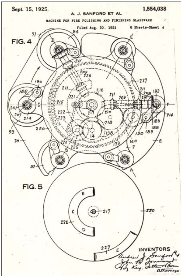
Patent 1,554,038 – Illustration 4
