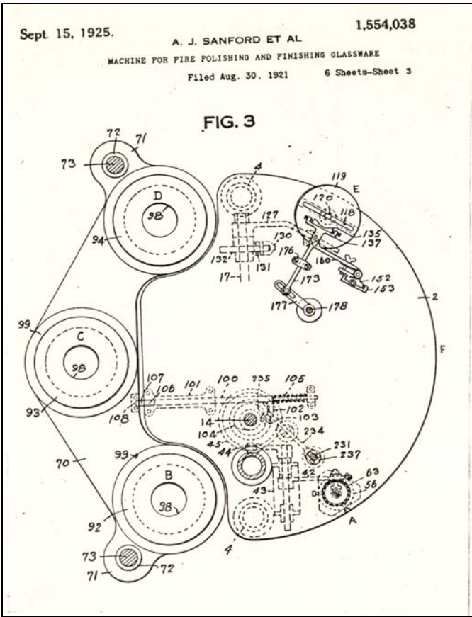
Patent 1,554,038 – Illustration 3
