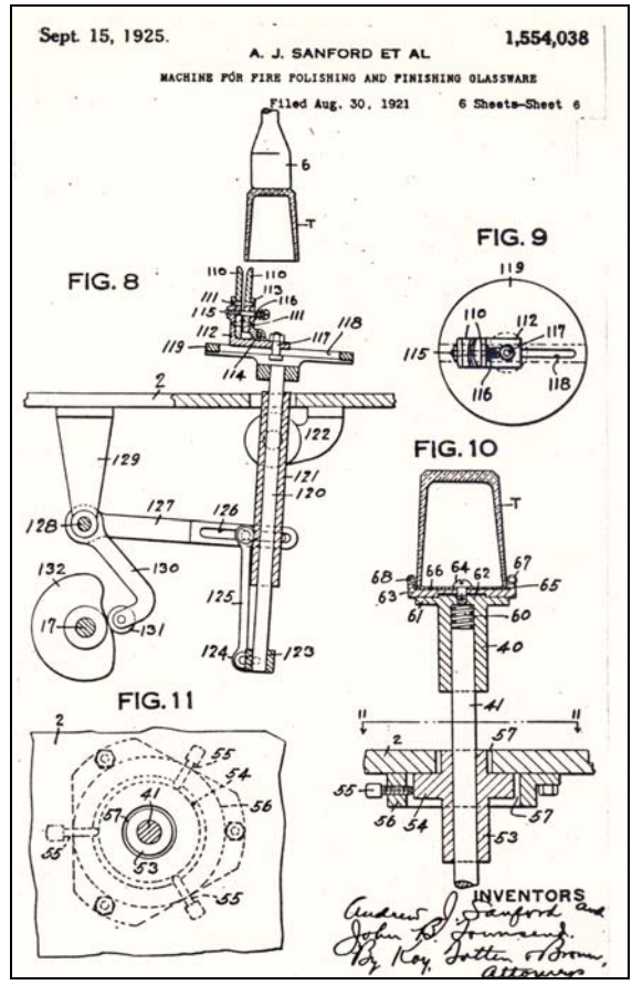
Patent 1,554,038 – Illustration 6
