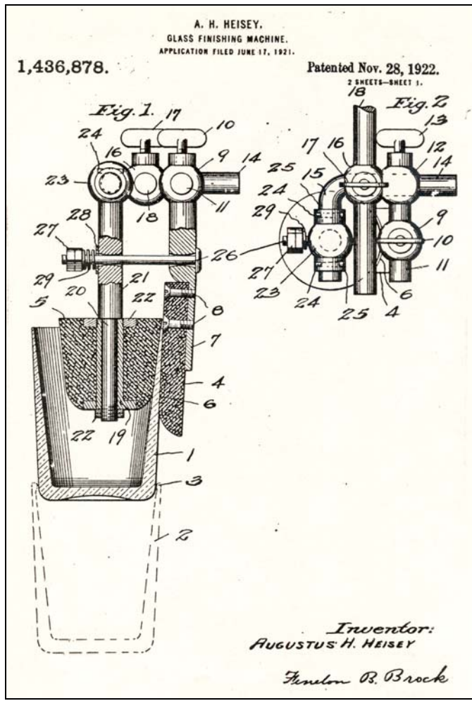
Patent 1,436,878 – Illustration 1
