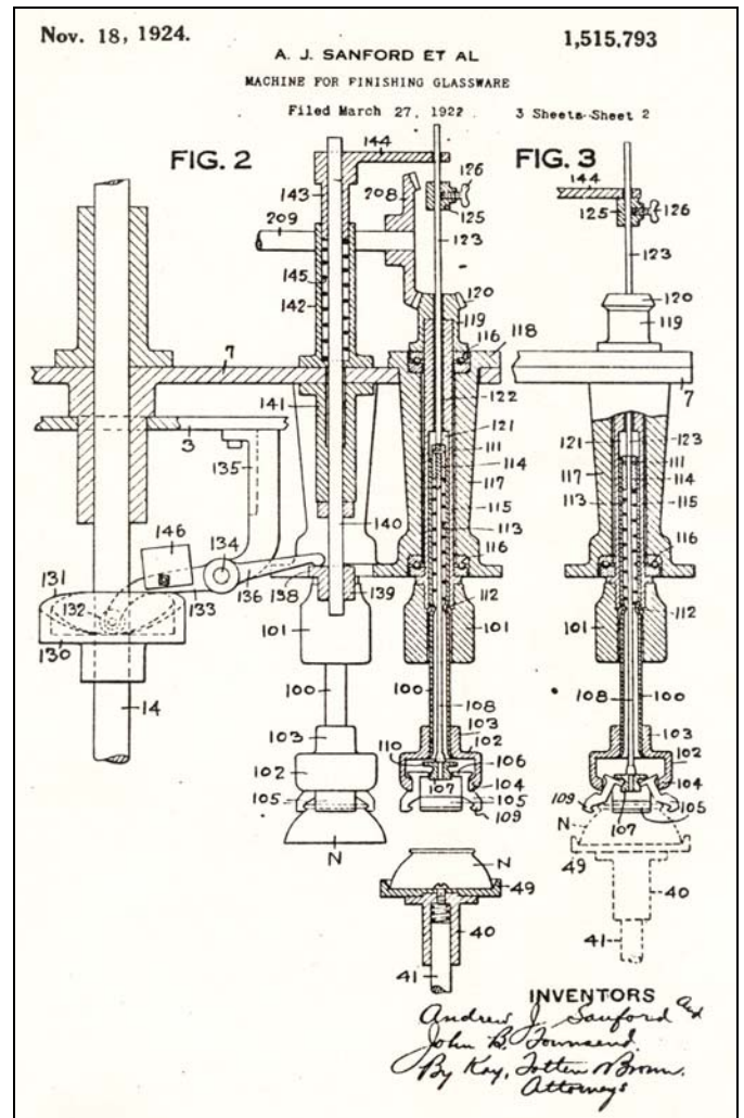
Patent 1,515,793 – Illustration 2
