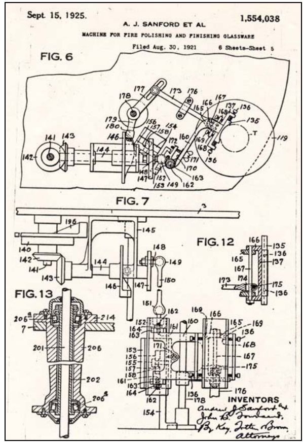
Patent 1,554,038 – Illustration 5
